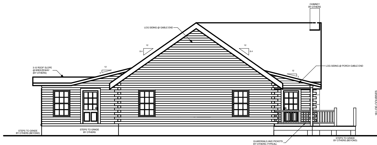
LEFT ELEVATION
