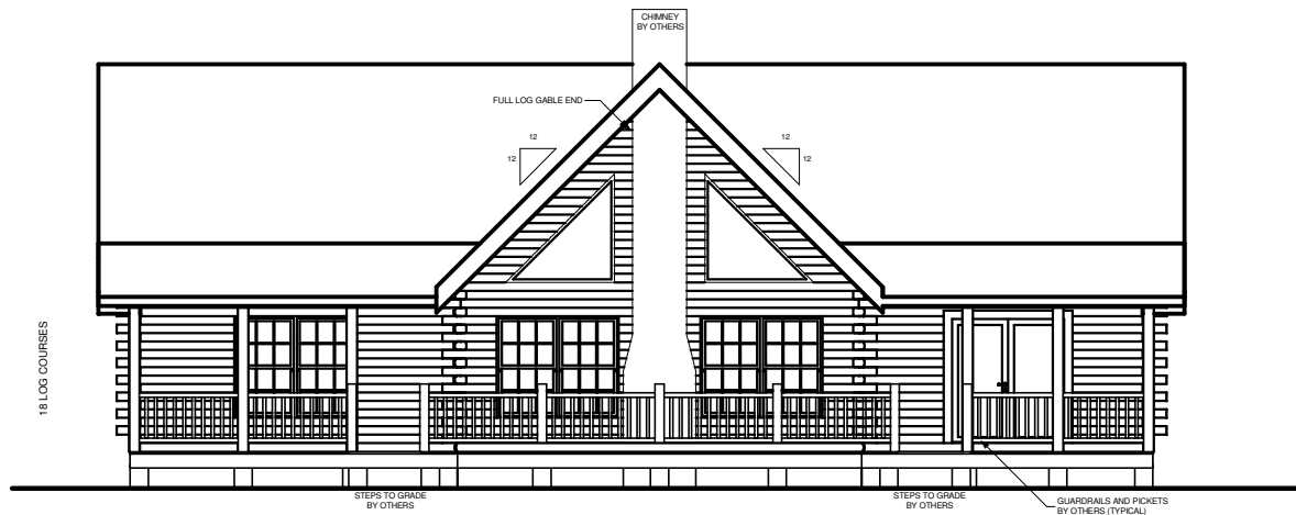
FRONT ELEVATION
