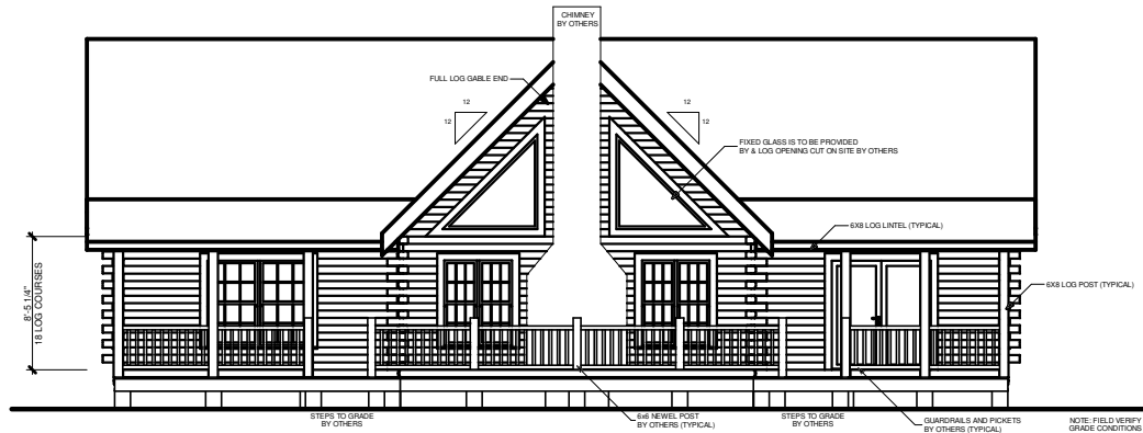
FRONT ELEVATION 1/4" = 1'-0"
