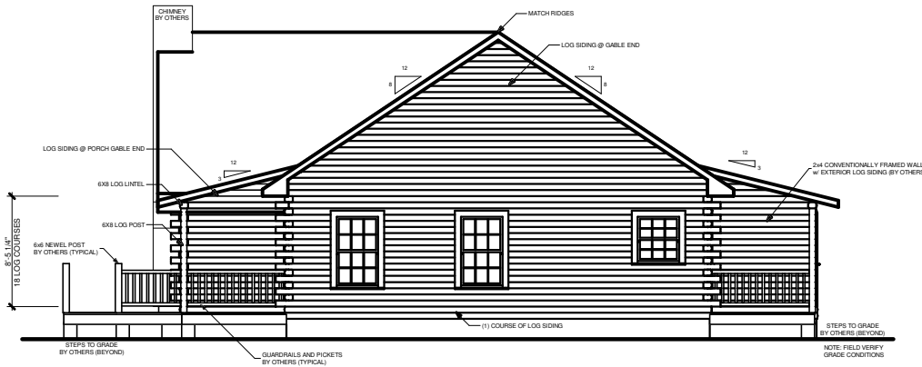
RIGHT ELEVATION 1/4" = 1'-0"
