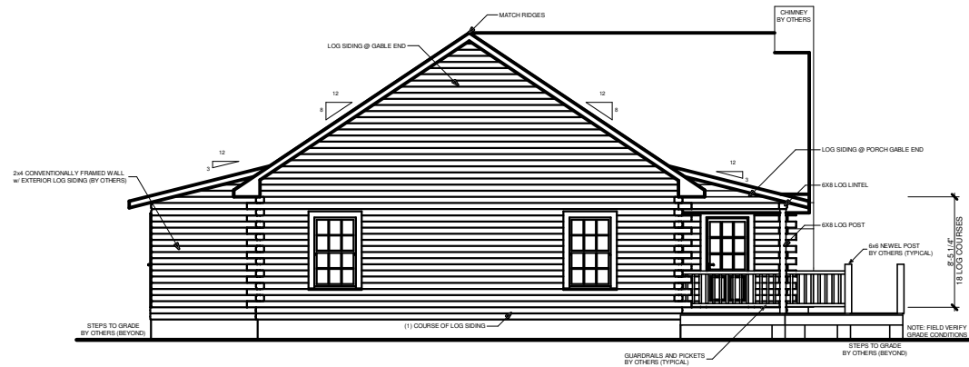
LEFT ELEVATION
