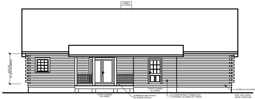
REAR ELEVATION 1/4" = 1'-0"
