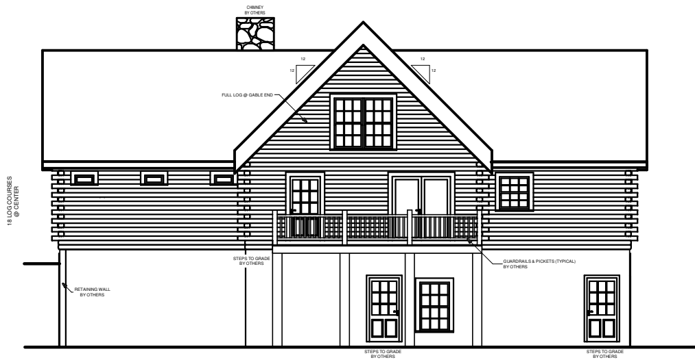
REAR ELEVATION
