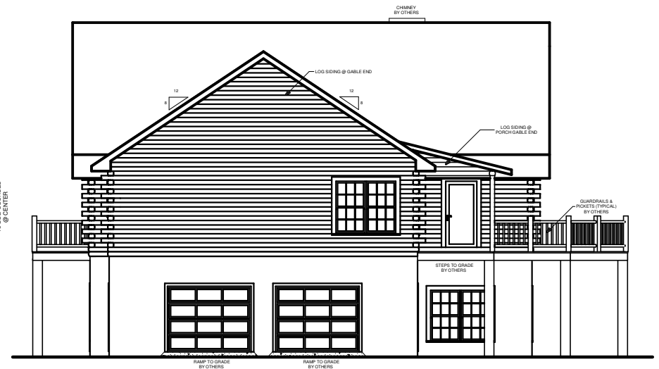
LEFT ELEVATION
