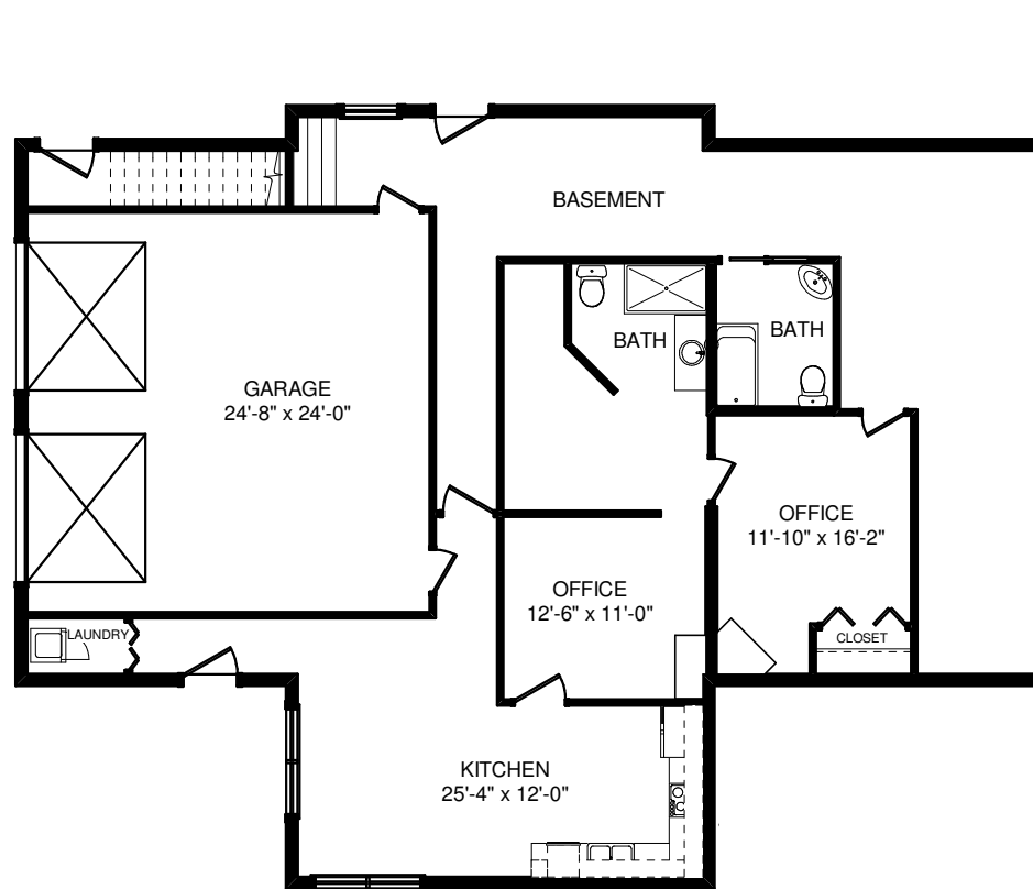
BASEMENT PLAN
