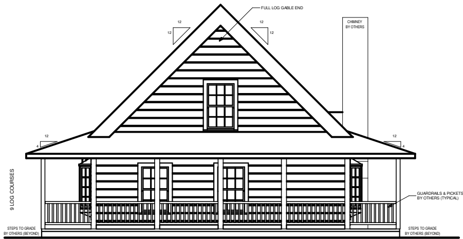
REAR ELEVATION
