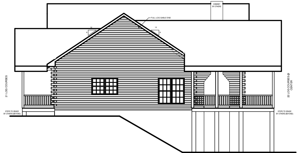
LEFT ELEVATION
