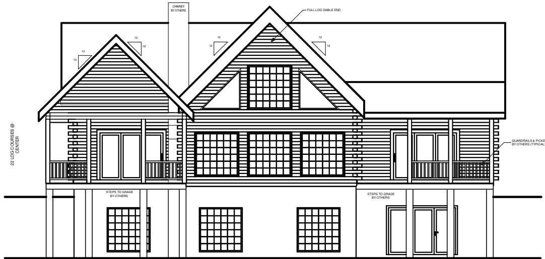
FRONT ELEVATION
