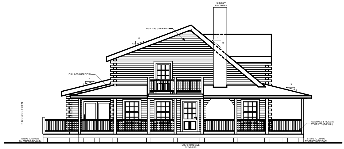
LEFT ELEVATION
