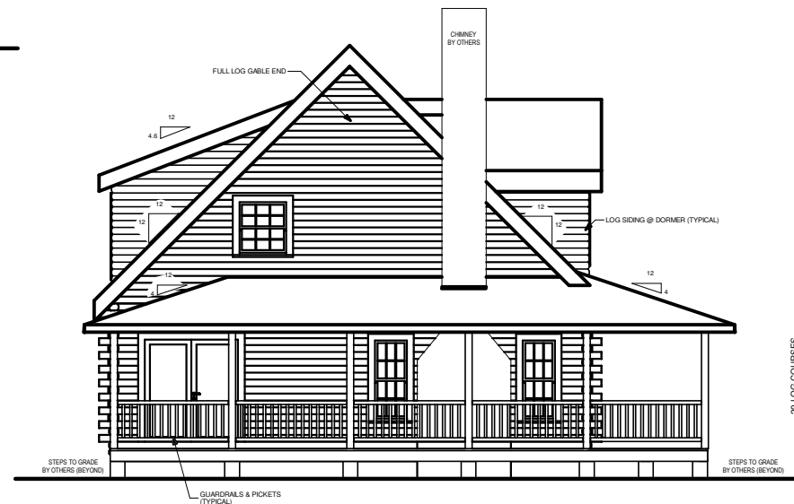
LEFT ELEVATION
