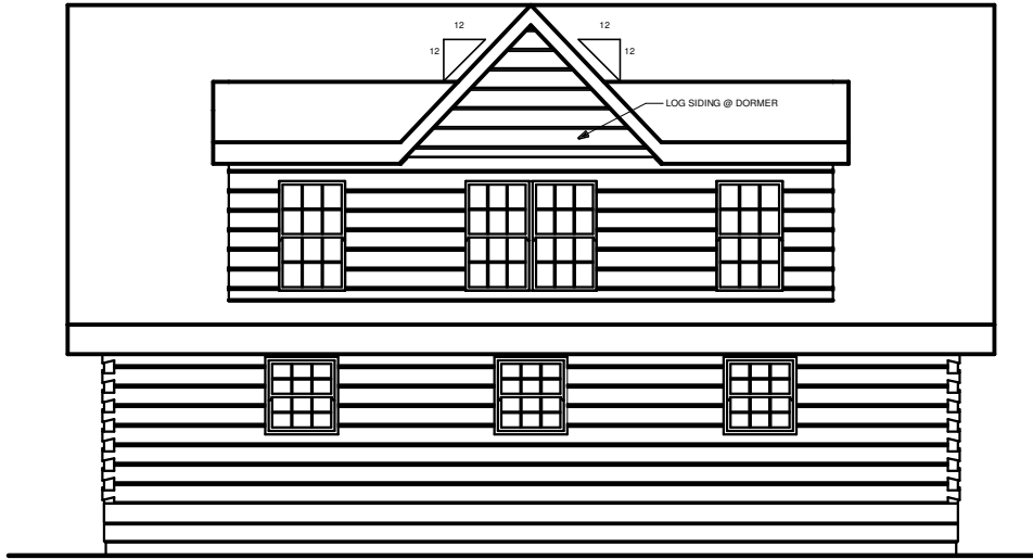
REAR ELEVATION
