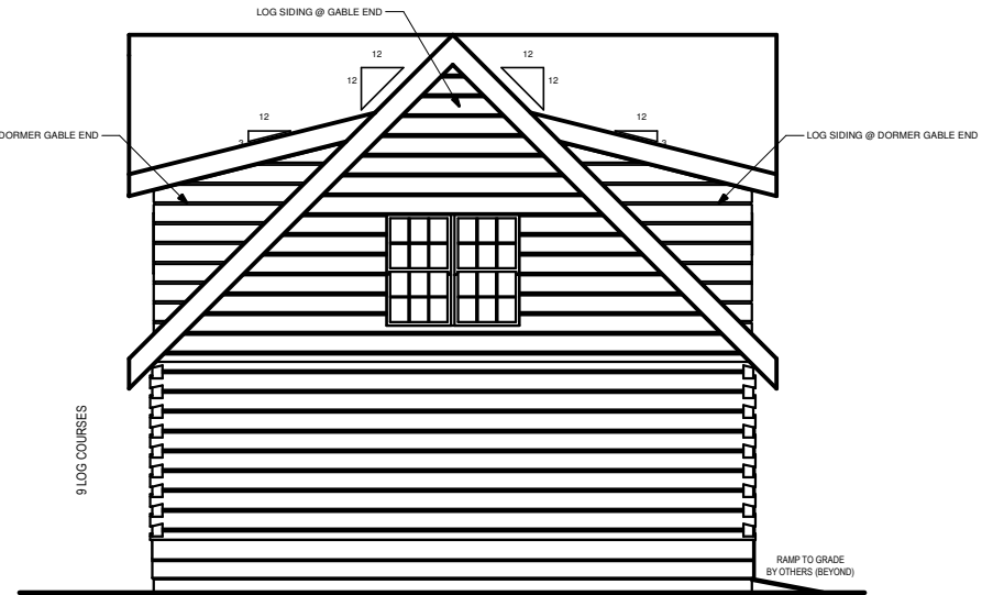
LEFT ELEVATION
