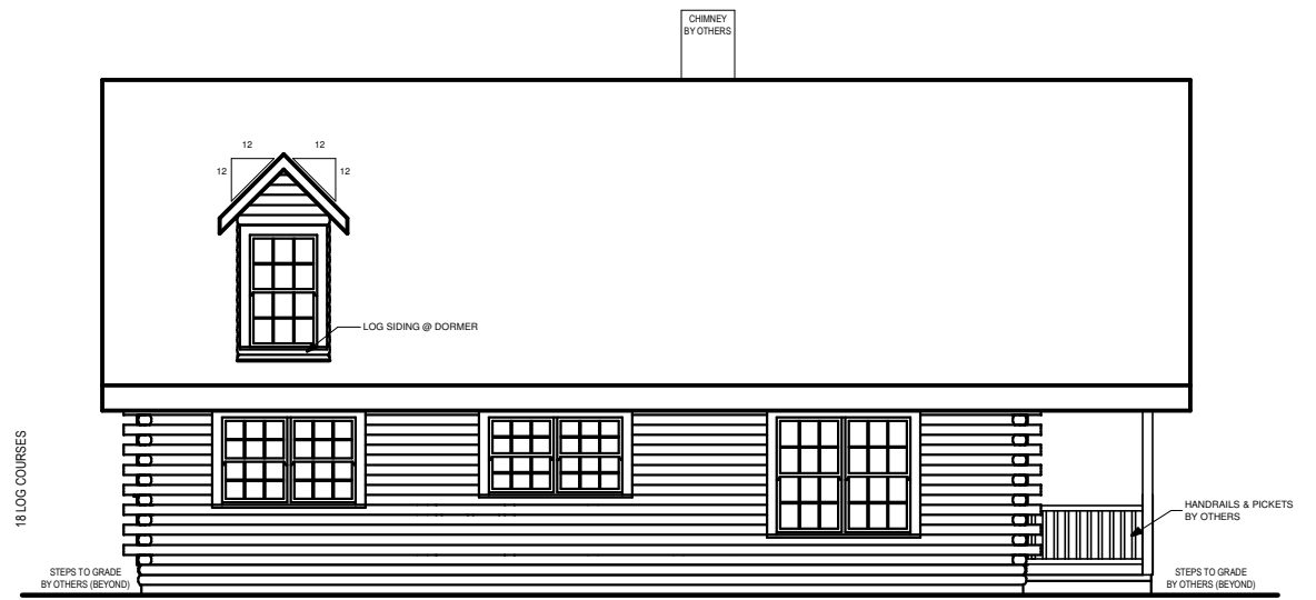
LEFT ELEVATION
