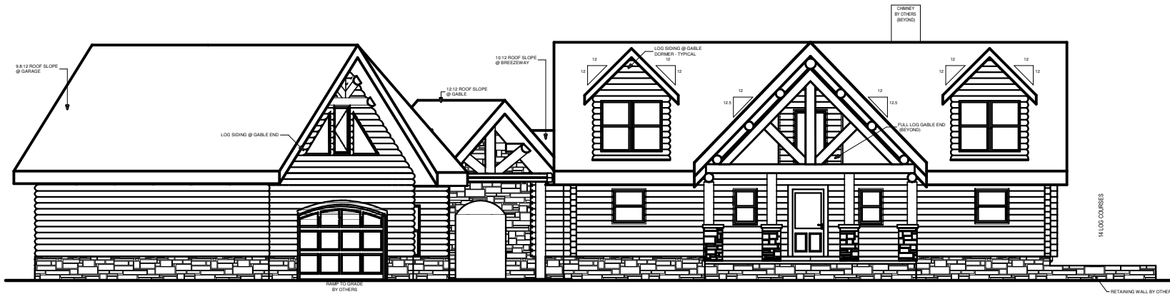
FRONT ELEVATION
