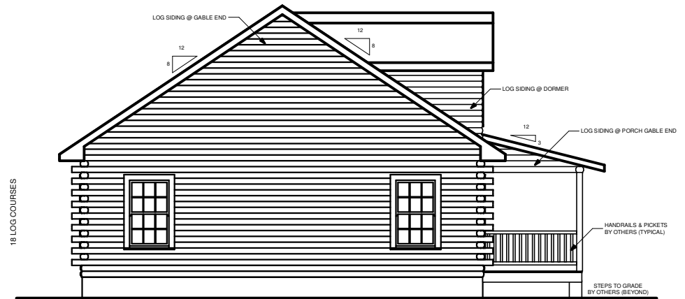
LEFT ELEVATION
