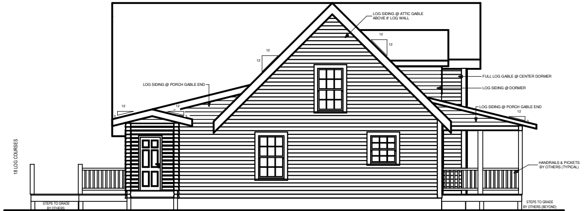
LEFT ELEVATION
