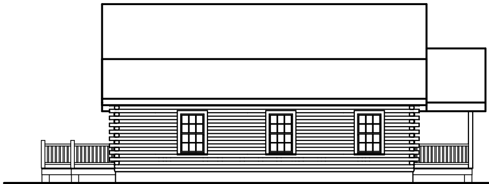
LEFT ELEVATION 16' x 1'0"
