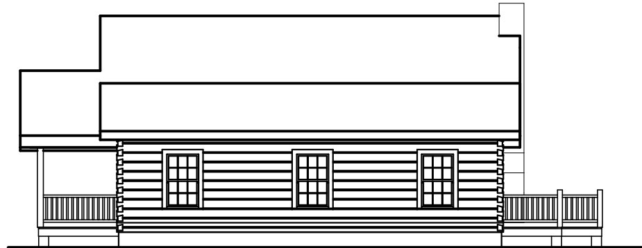
RIGHT ELEVATION 1/4" = 1'-0"
