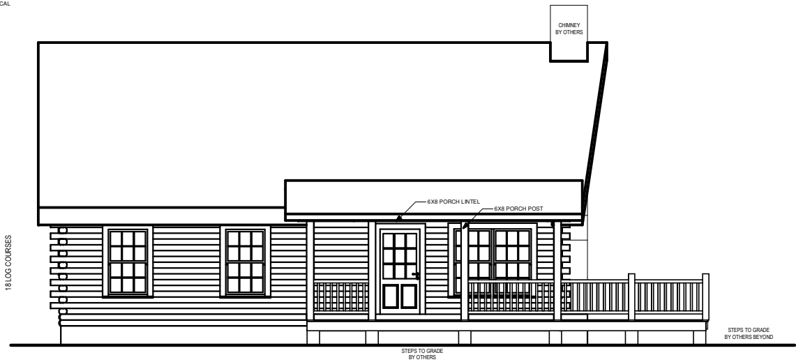
LEFT ELEVATION
