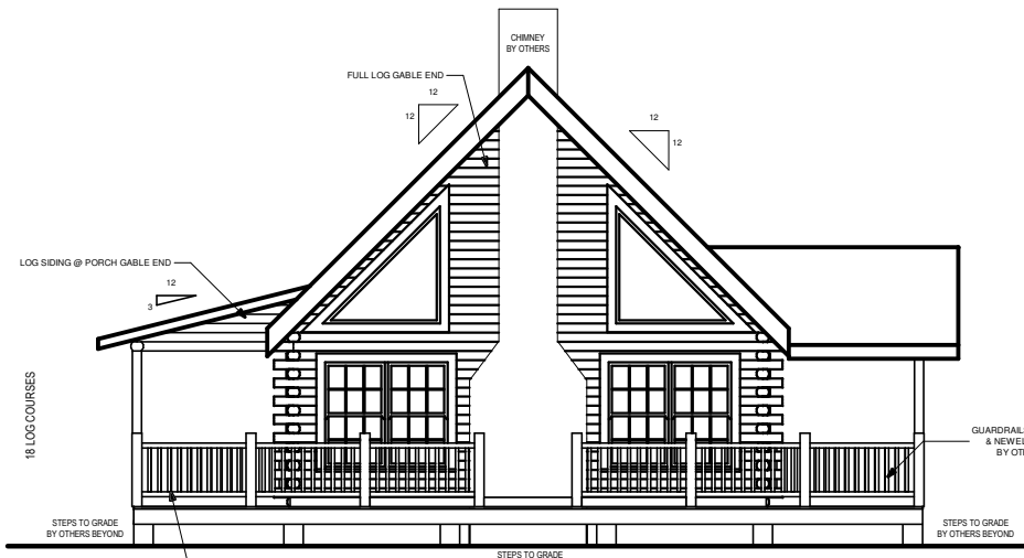
FRONT ELEVATION
