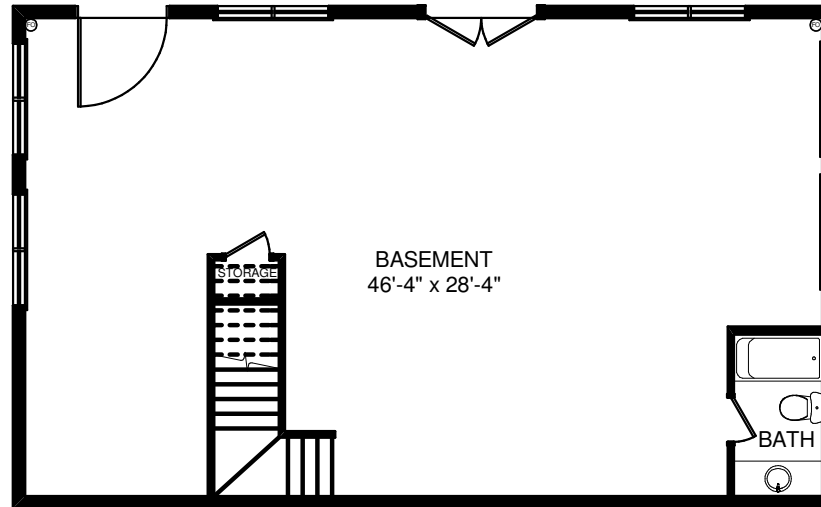
BASEMENT PLAN
