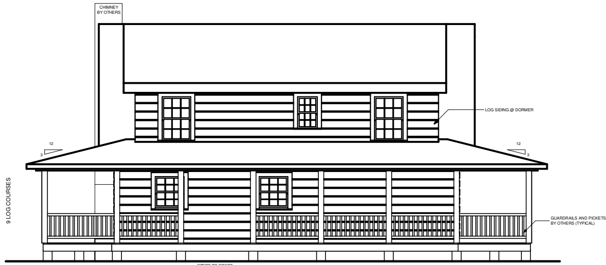
REAR ELEVATION
