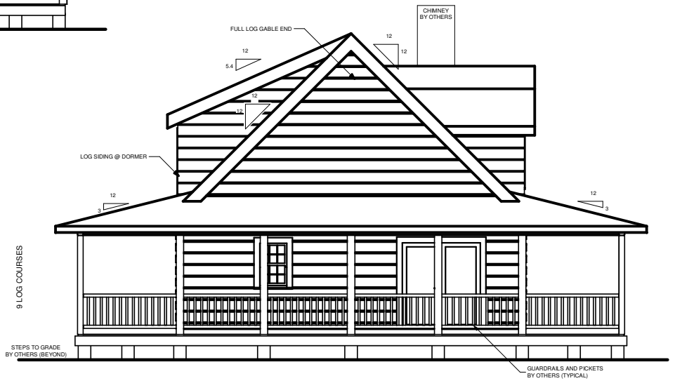
LEFT ELEVATION
