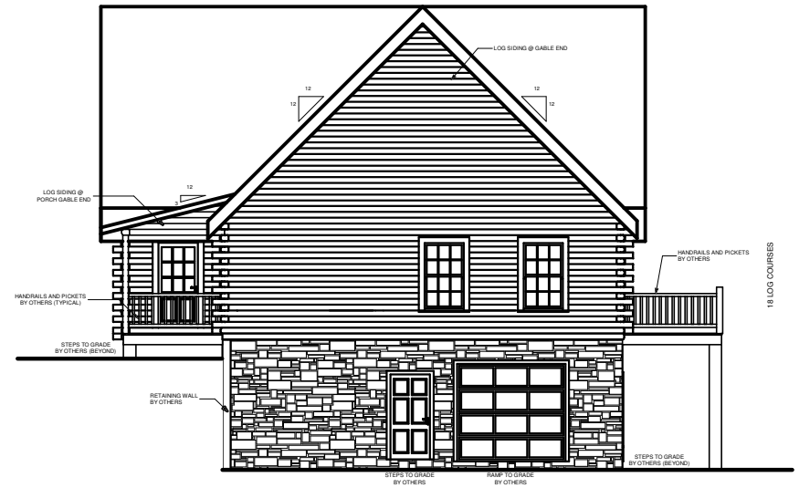
LEFT ELEVATION
