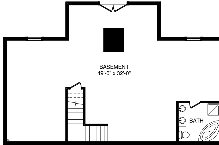
BASEMENT PLAN
