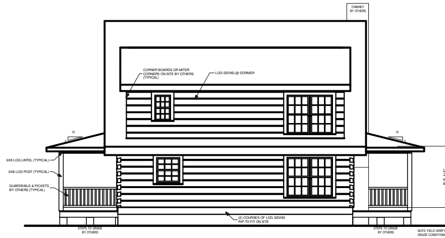
REAR ELEVATION
