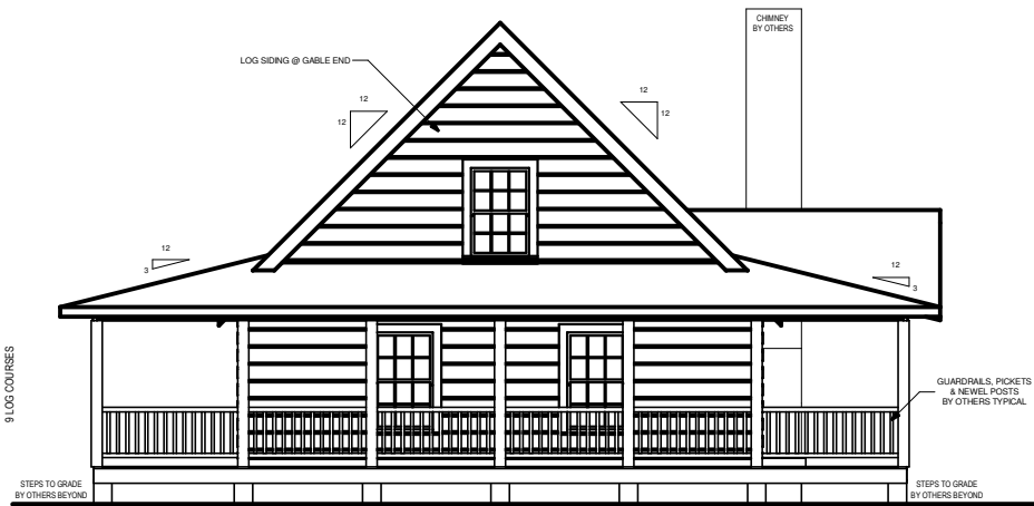
REAR ELEVATION
