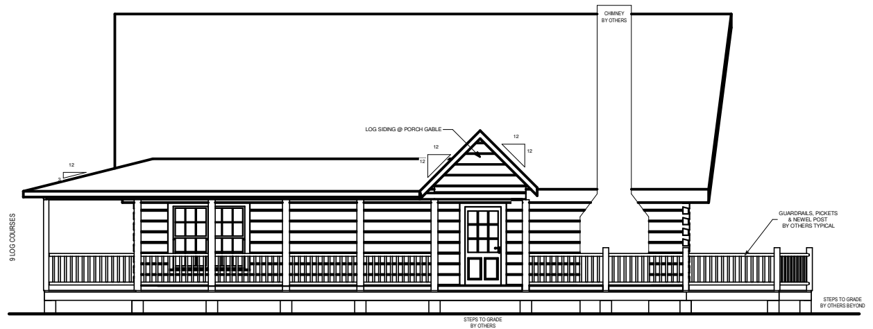
LEFT ELEVATION
