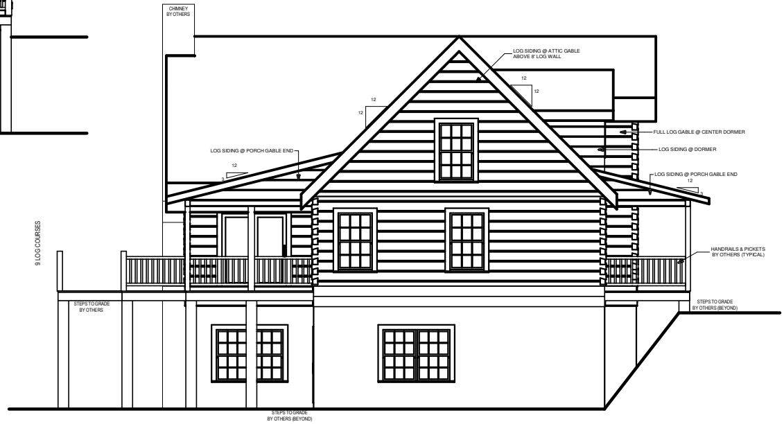
LEFT ELEVATION
