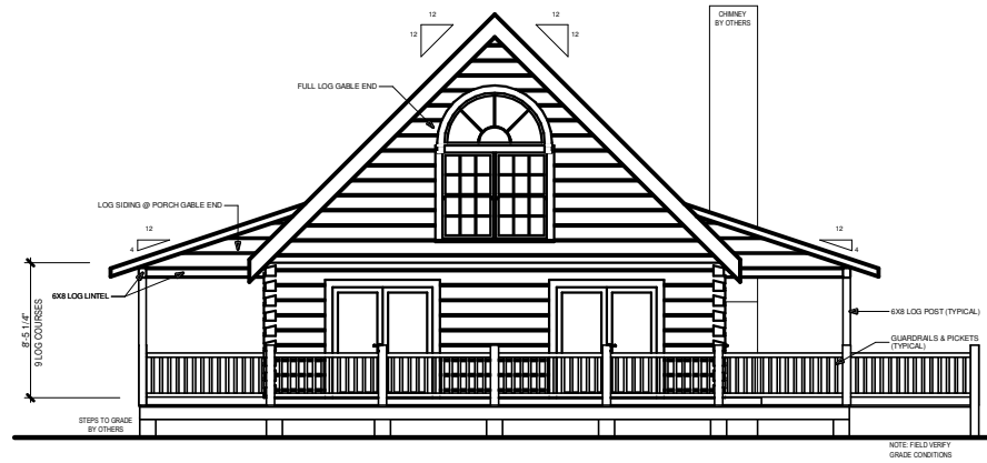
REAR ELEVATION 1/4" = 1'-0"
