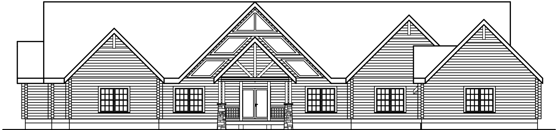
FRONT ELEVATION
