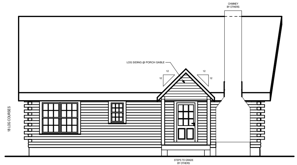
LEFT ELEVATION
