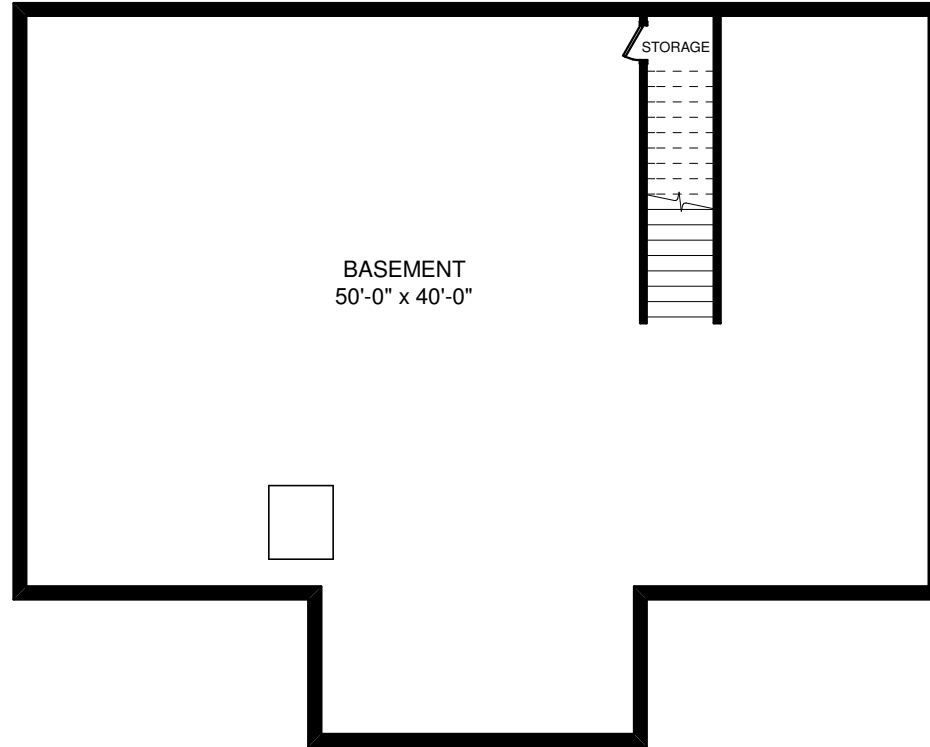
BASEMENT PLAN
