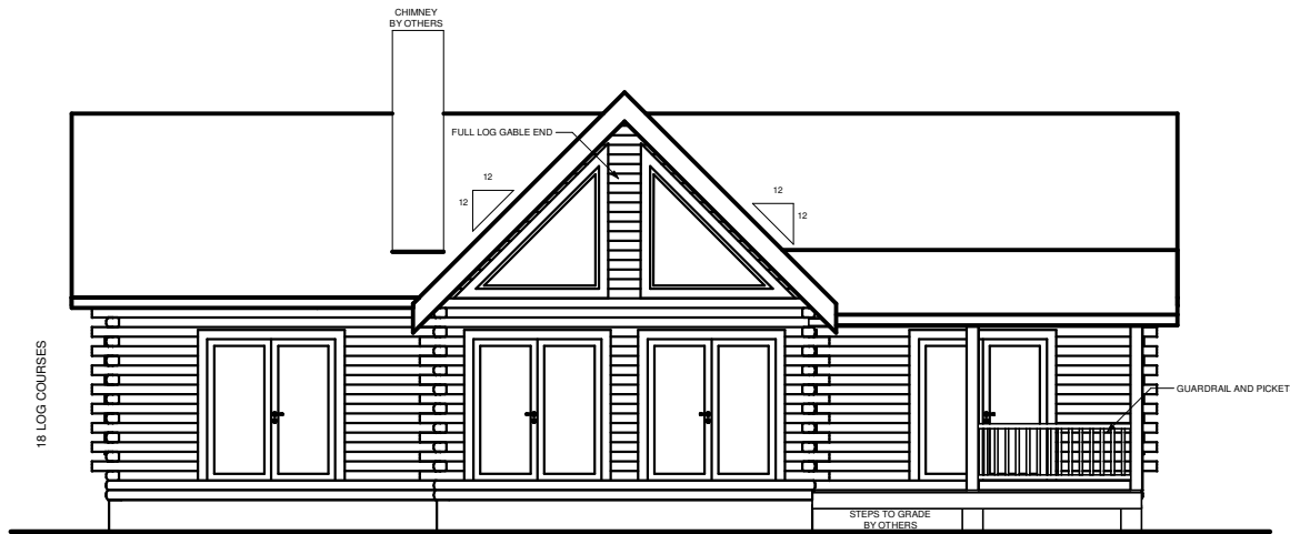
FRONT ELEVATION
