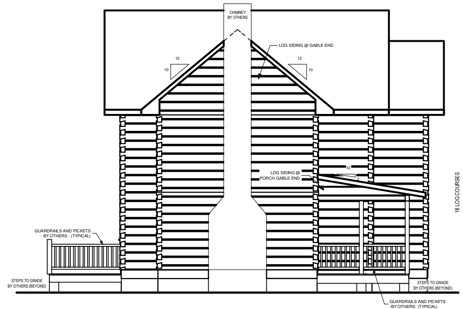
LEFT ELEVATION
