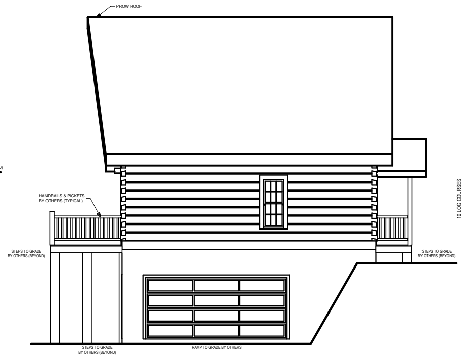
LEFT ELEVATION
