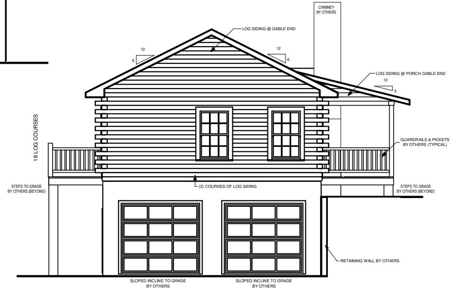
LEFT ELEVATION
