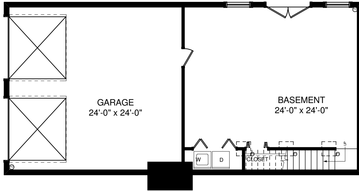
BASEMENT PLAN
