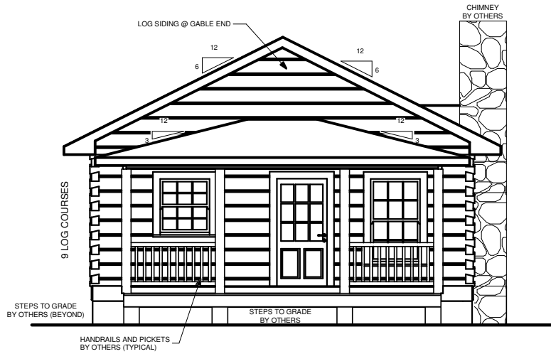
FRONT ELEVATION
