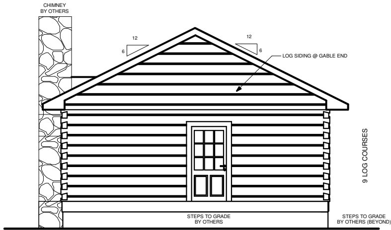
REAR ELEVATION
