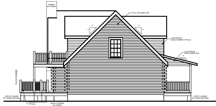
LEFT ELEVATION
