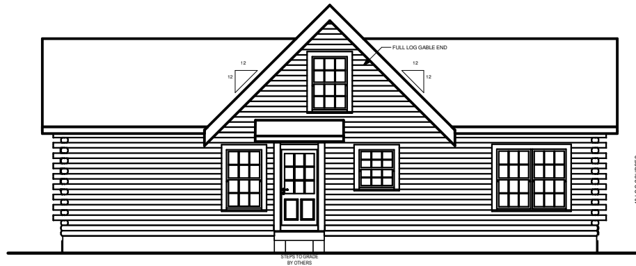
REAR ELEVATION
