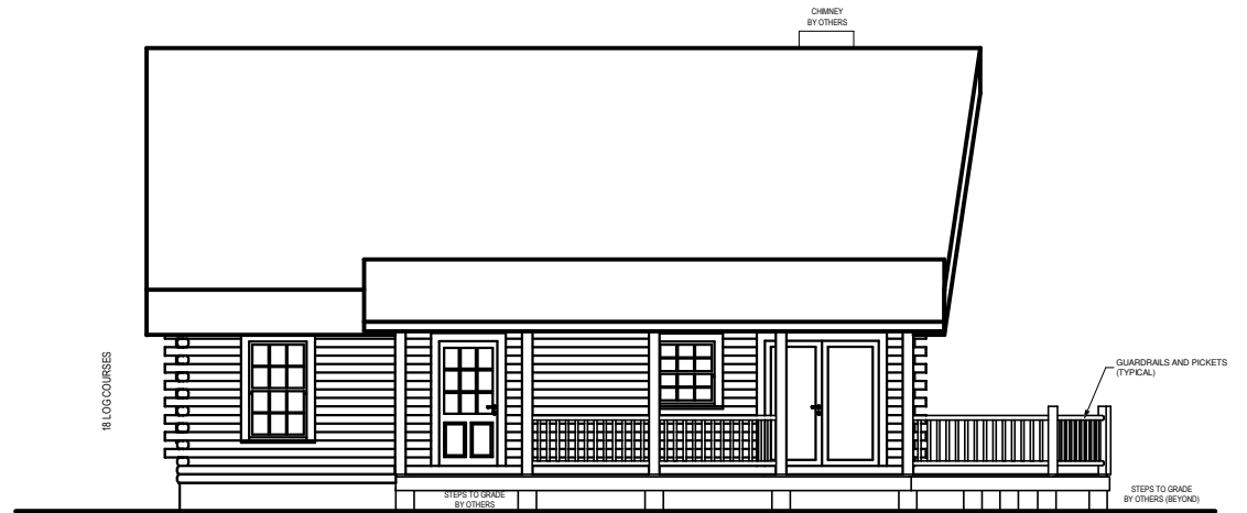
LEFT ELEVATION
