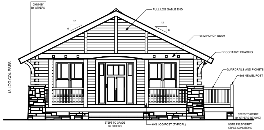
FRONT ELEVATION
