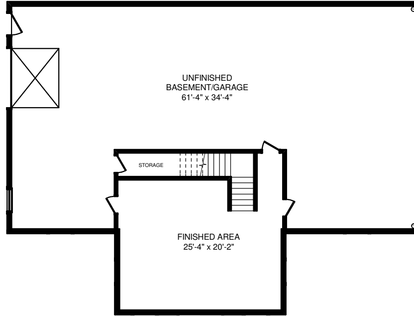
BASEMENT PLAN
