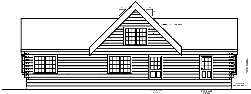
REAR ELEVATION
