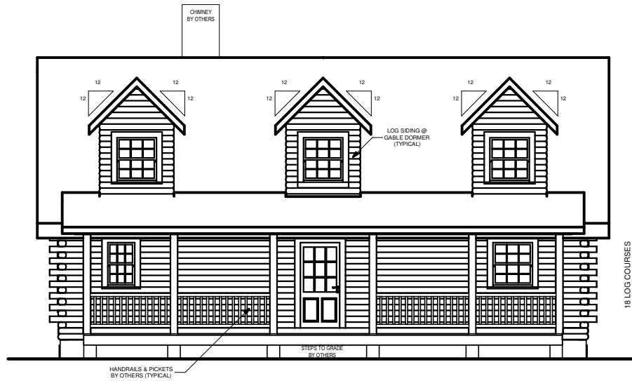
FRONT ELEVATION
