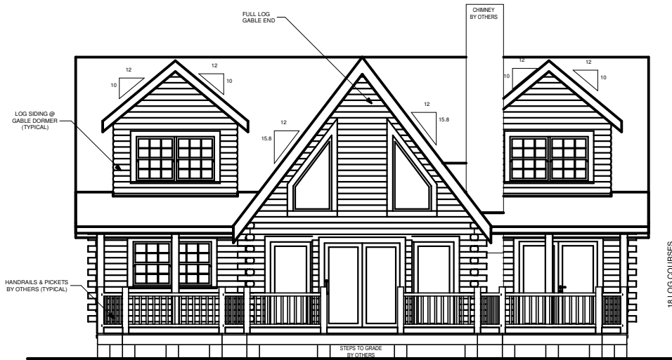
REAR ELEVATION
