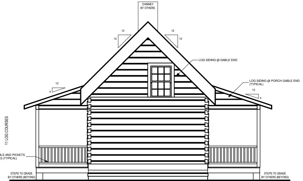
LEFT ELEVATION
