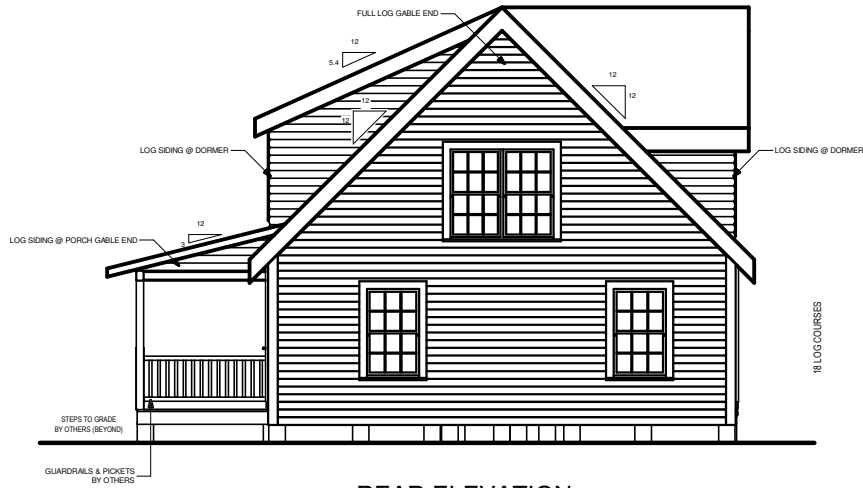
REAR ELEVATION
