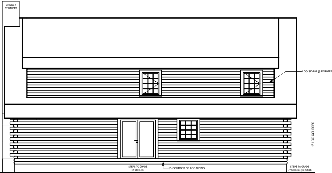
REAR ELEVATION
