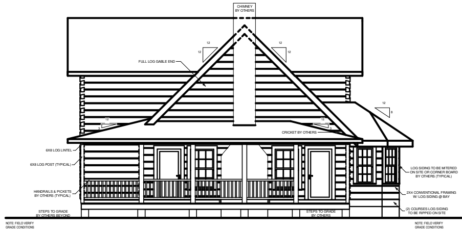
RIGHT ELEVATION 1/4" = 1'-0"
