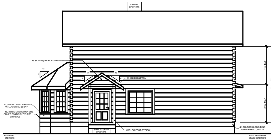
LEFT ELEVATION
