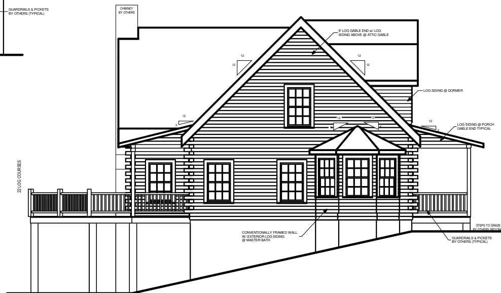
LEFT ELEVATION
