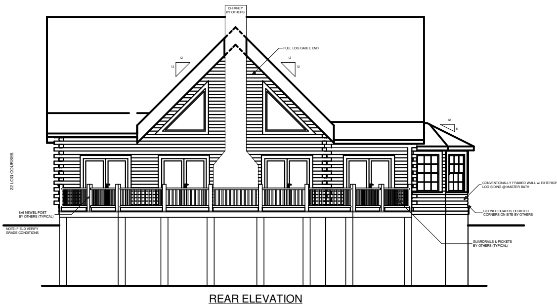
REAR ELEVATION
