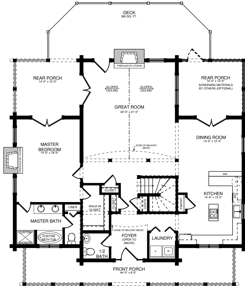
FIRST FLOOR PLAN 1/4" = 1'-0"
