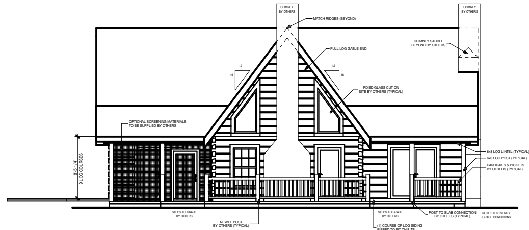
REAR ELEVATION 1/4" = 1'-0"
