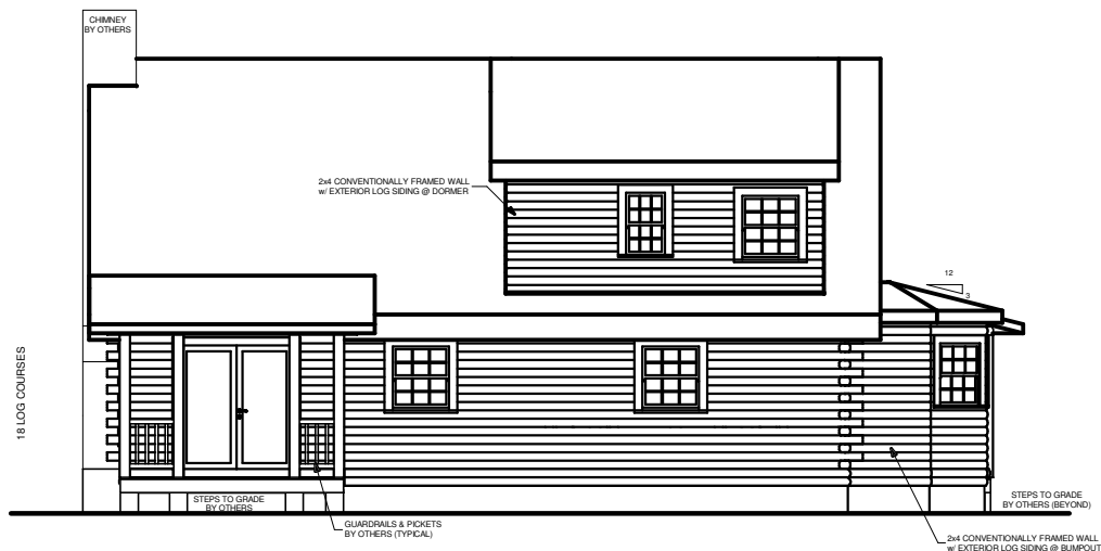
REAR ELEVATION
