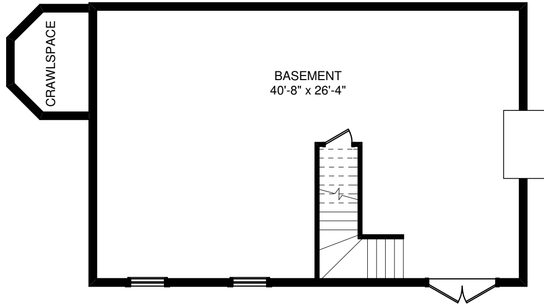
BASEMENT PLAN
