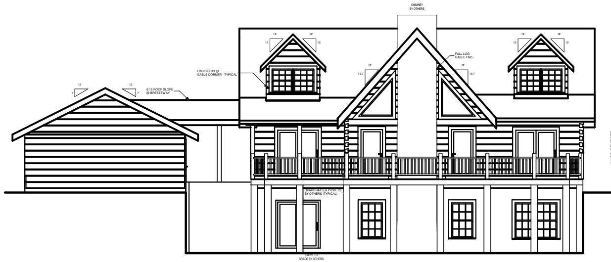
REAR ELEVATION
