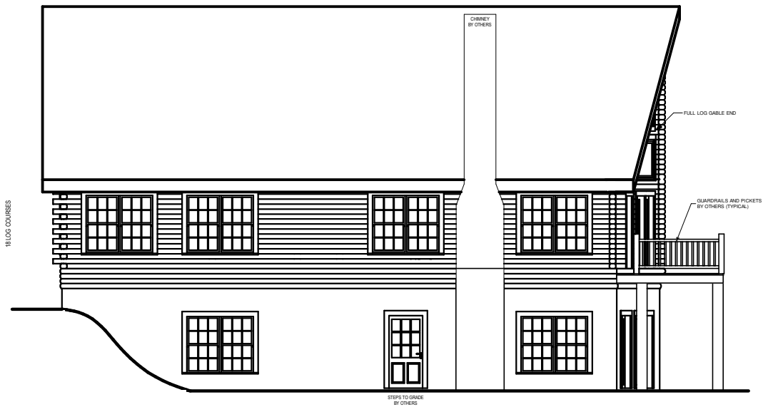
LEFT ELEVATION
