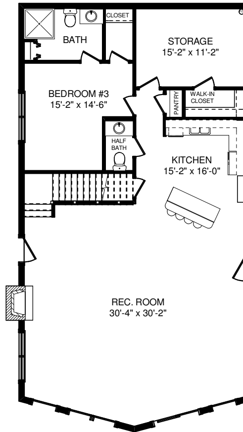
BASEMENT PLAN
