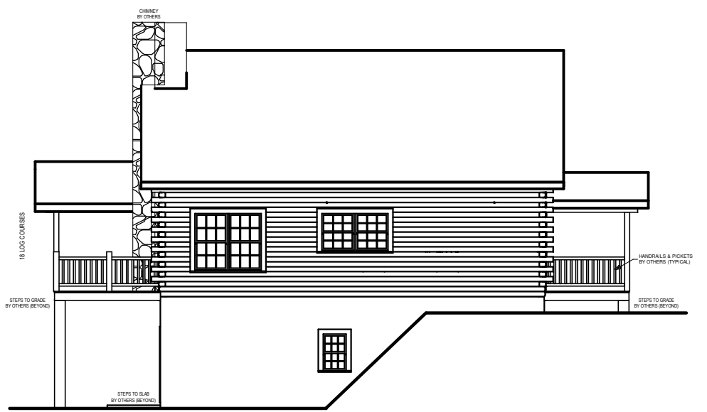
LEFT ELEVATION
