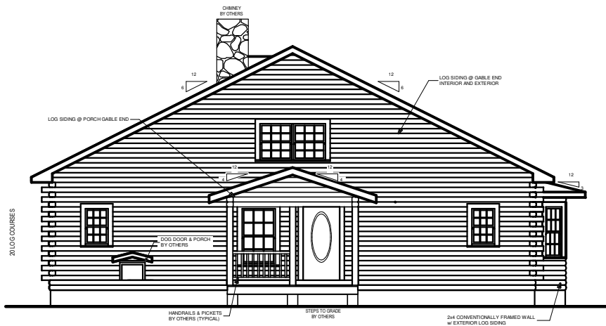
FRONT ELEVATION
