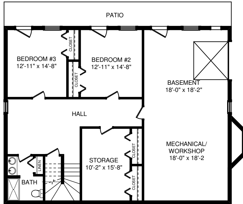
BASEMENT PLAN
