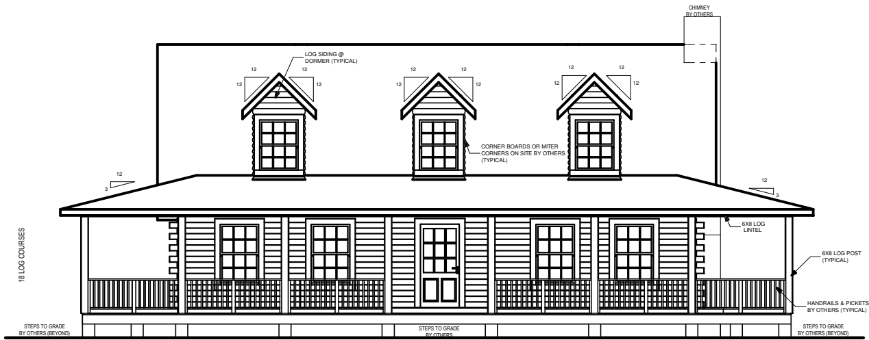
FRONT ELEVATION
