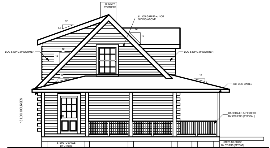
LEFT ELEVATION
