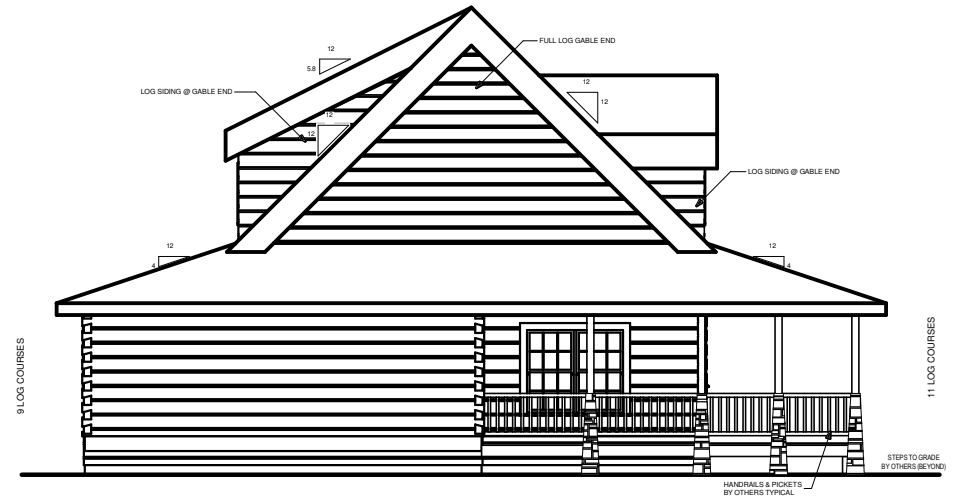
LEFT ELEVATION
