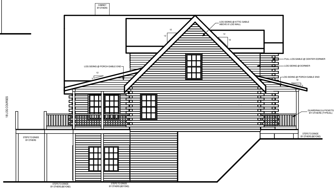
LEFT ELEVATION
