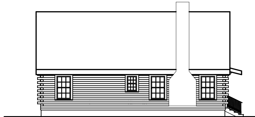
LEFT ELEVATION
